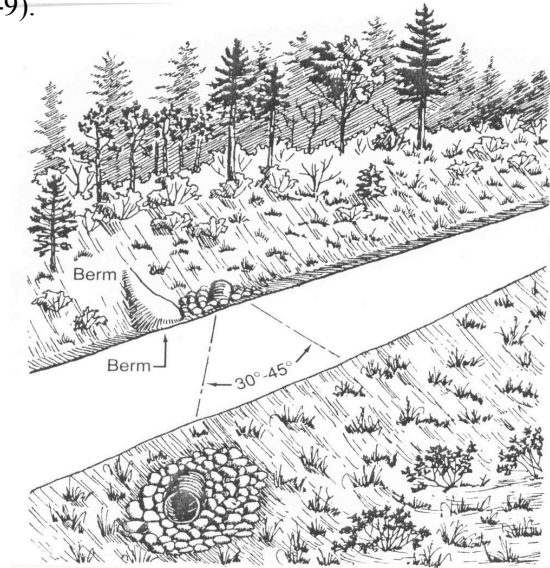
Figure 5-9. Cross-drain culvert.
