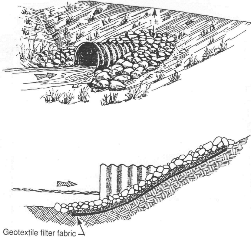
Figure 5-7. Use riprap around the inlet of culverts. Also use geotextile filter fabric for permanent installations.
