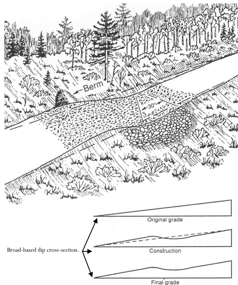
Figure 5-11. Broad-based dip.
